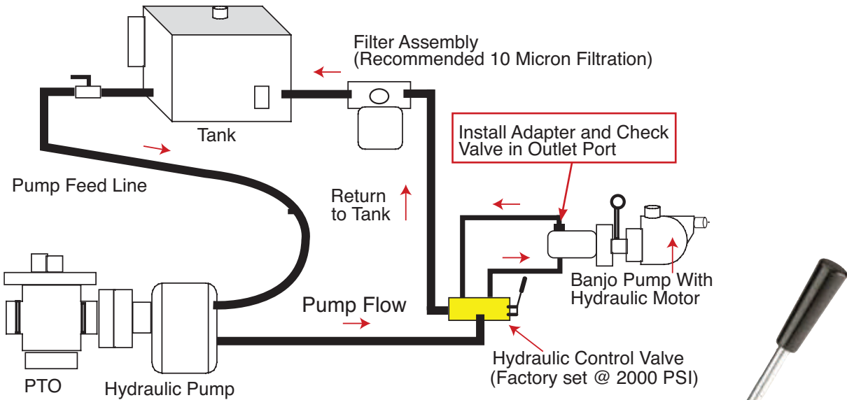
SPOOL VALVE ASSEMBLY DIAGRAM
